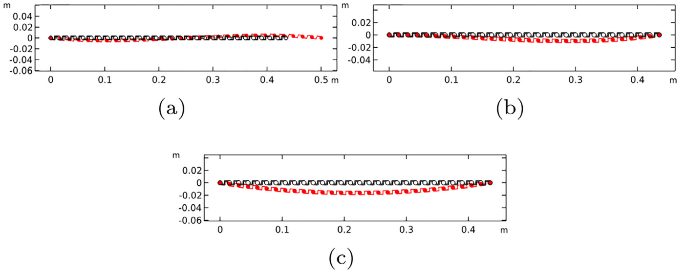
Fig. 5. Deformed shapes of Cauchy continuum model of the 2D granular system for (a) Identification Test 1, (b) Identification Test 2 and (c) Identification Test 3.
