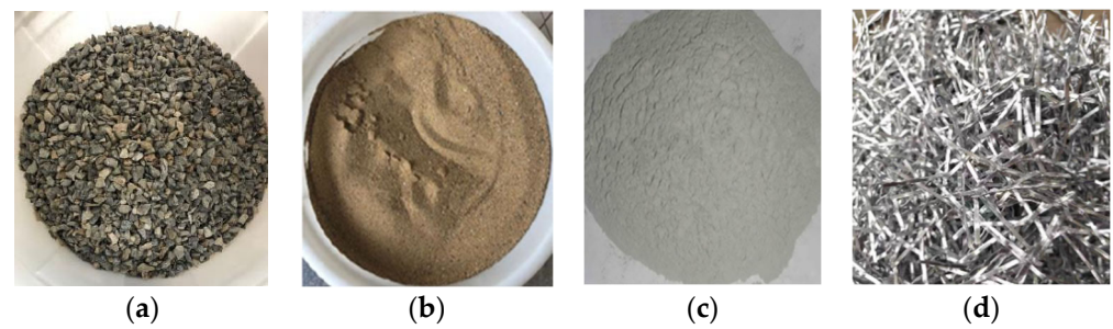
Figure 4. Main components of SFRC: (a) Aggregate; (b) Sand; (c) Cement; and (d) Steel fibres.
