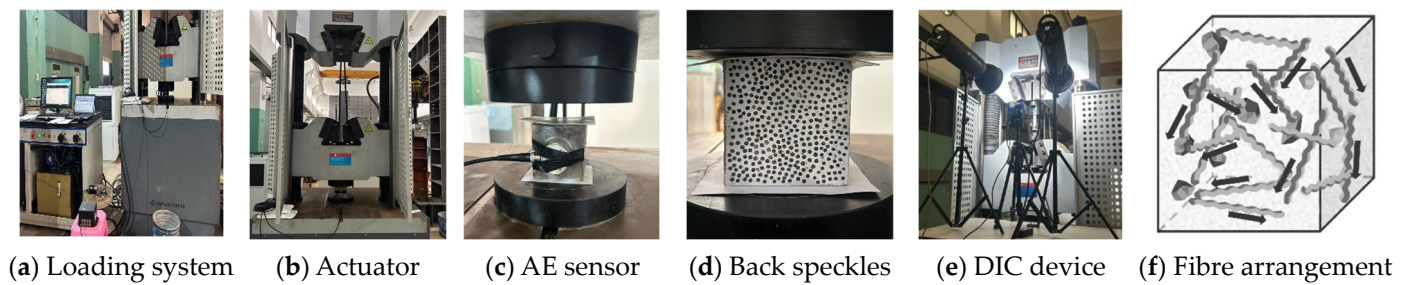
Figure 6. Test setup.
