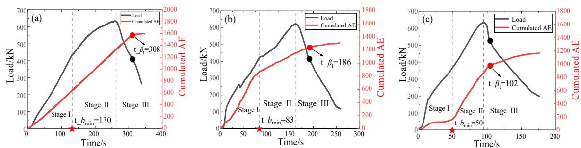
Figure 17. Cumulated AE and loading history at loading rates of (a) 0.4 mm/min, (b) 0.8 mm/min, and (c) 1.2 mm/min.
