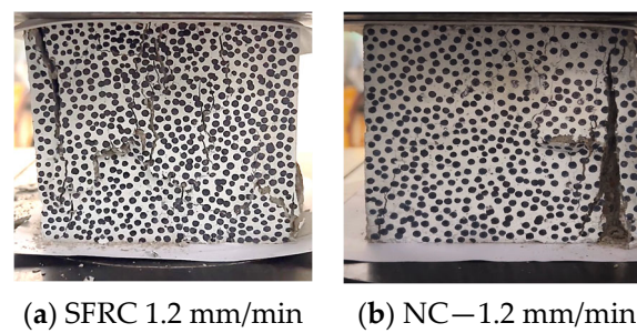
Figure 15. Comparison of SFRC and NC sample failures.
