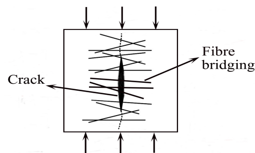
Figure 1. Bridging mechanism of fibre reinforcements.
