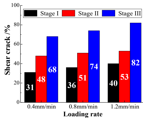
Figure 19. Shear cracks in each damage stage and at different loading rates.
