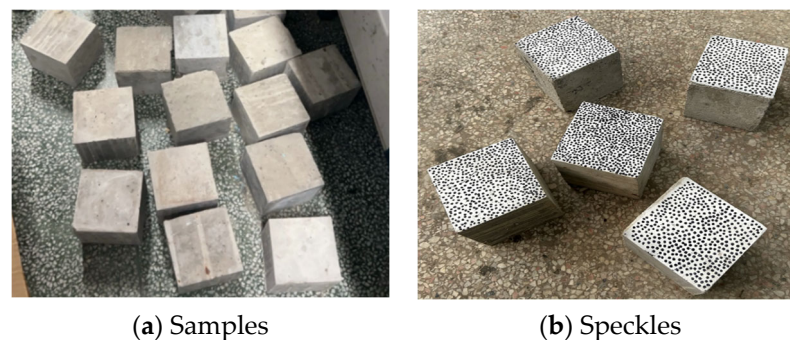
Figure 5. Overview of test samples.
