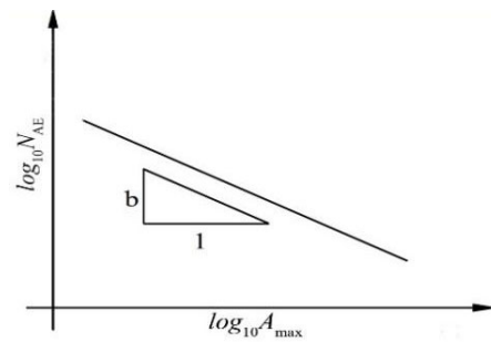
Figure 8. GR's law and AE events.
