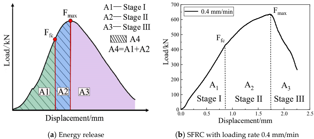
Figure 11. SFRC compressive toughness.
