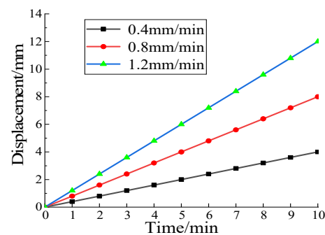
Figure 7. Loading regimes.
