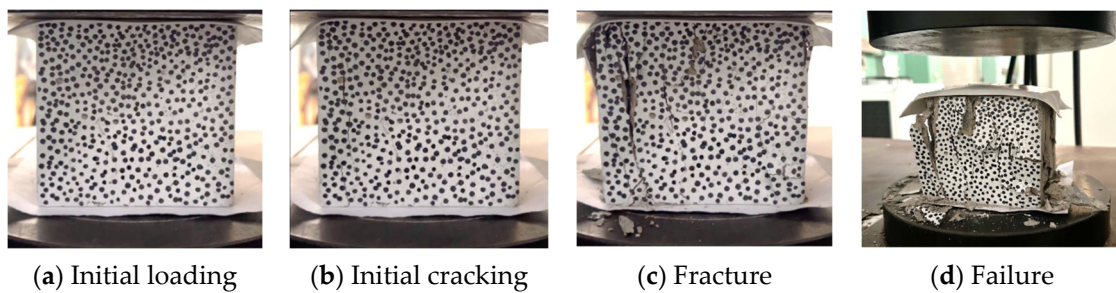
Figure 12. SFRC damage evolution (loading rate: 0.4 mm/min).
