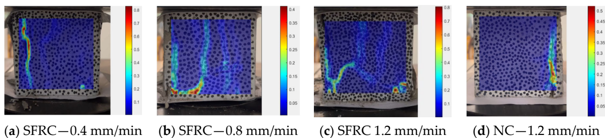
Figure 14. DIC strain analysis at fracturing with different loading rates.
