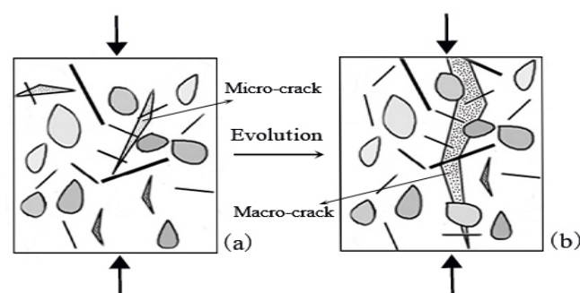
Figure 2. Micro- and macro-cracks bridged by fibres. (a) Micro-crack stage; (b) Macro-crack stage.
