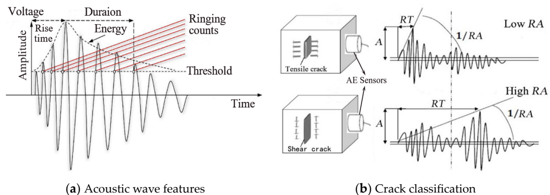
Figure 9. Crack type and AE.
