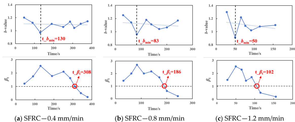
Figure 16. \beta_t and b -values at different loading rates.
