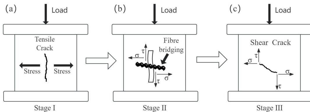
Figure 20. Tensile-to-shear crack transition. (a) Stage I; (b) Stage II; (c) Stage III.
