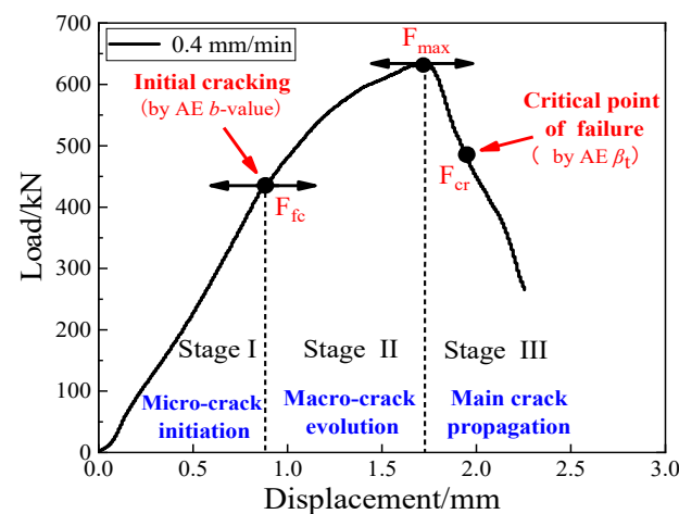
Figure 10. Load–displacement curve with indicated three stages.
