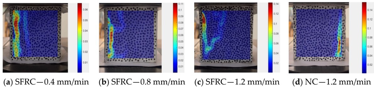
Figure 13. DIC strain analysis at initial cracking with different loading rates.
