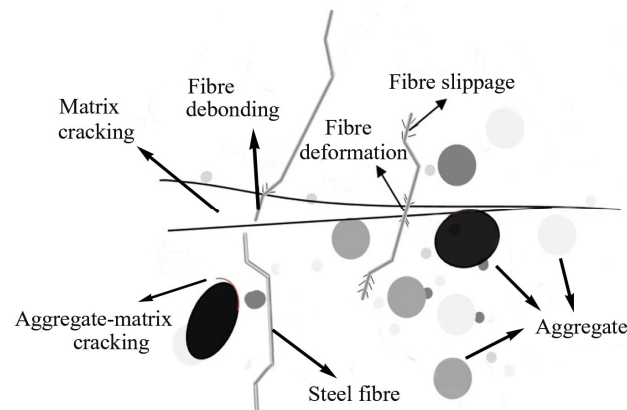
Figure 3. Meso-scale damage of SFRC.
