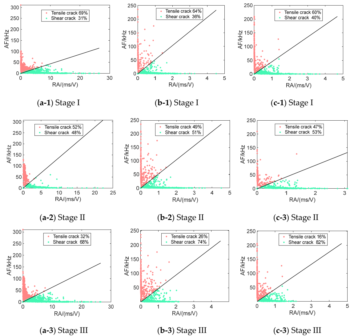
Figure 18. AF and RA in SFRC samples: (a-1–a-3) 0.4 mm/min, (b-1–b-3) 0.8 mm/min, and (c-1–c-3) 1.2 mm/min.
