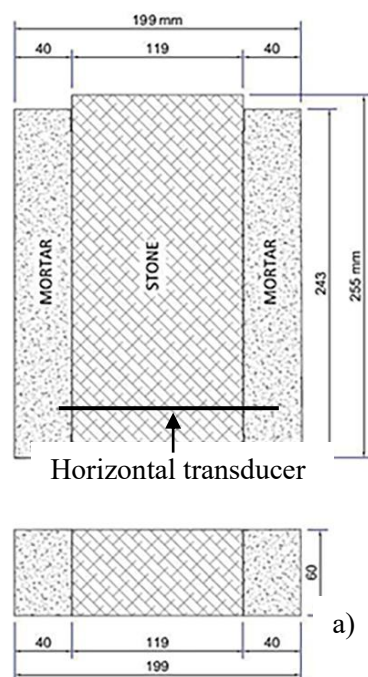
Figure 2. Geometry of composite specimen (a) and test setup (b).
