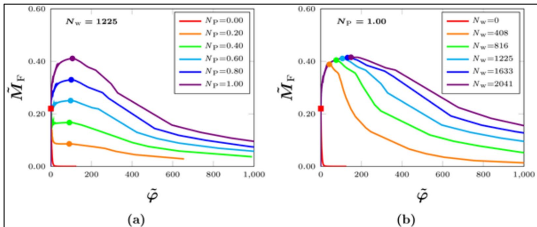
Fig. 5 Size-scale effects in FRC beams. The dimensionless moment of first fracturing is represented by the red square. a: Different flexural responses by varying N_p . The minimum reinforcement condition occurs when N_p = 0.6 (light-blue curve); b: Different flexural responses by varying N_w . The plastic rotation capacity increases by increasing N_w
