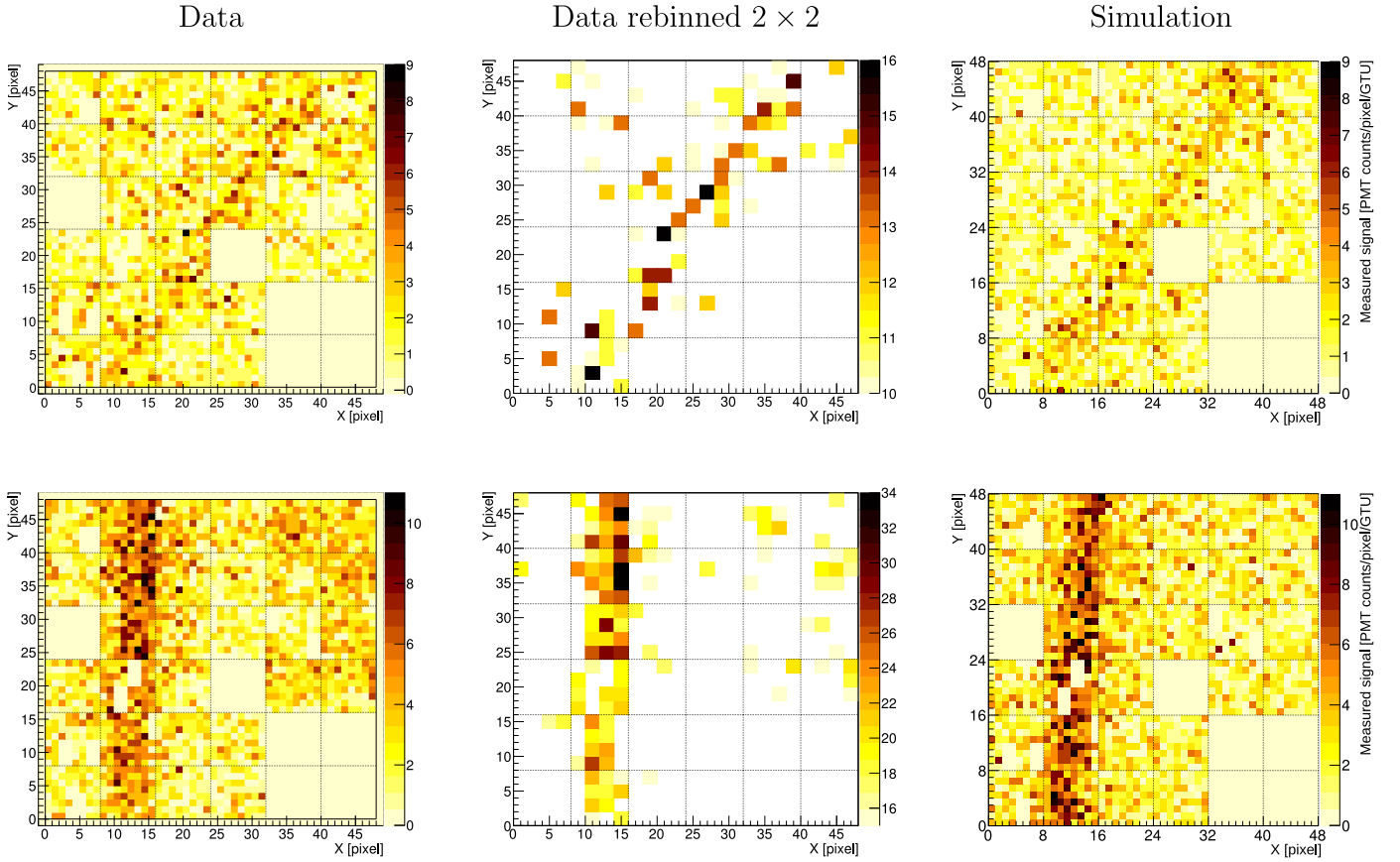
Fig. 21. Two out of the 9 UHECR observed by EUSO-TA. The left plot shows the real data in photoelectron counts, in the centre 2 \times 2 rebinning of the data is shown and in the right plot the simulation made with the OffLine package. The top panels are for an event of energy of 10^{18} eV, impact parameter 2.5 km with respect to the telescope, zenith angle of the axis of 35^\circ and azimuth angle of 7^\circ . The bottom panels correspond to an energy of 10^{18.4} eV, impact parameter 2.6 km, zenith angle of the axis of 8^\circ and azimuth angle of 82^\circ .
