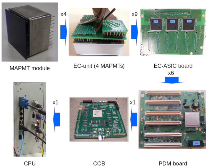
Fig. 5. Scheme of the signal flow in the EUSO-TA experiment. The labels over arrows denote signal from how many subsystems of the previous level is included in the subsystem of the next level.
