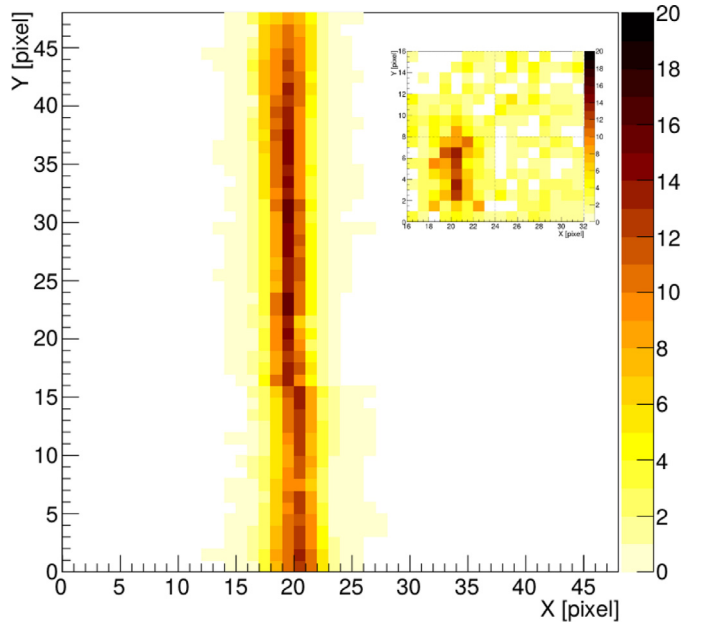
Fig. 14. An average of 259 tracks of the CLF laser, for a telescope elevation angle of 10^\circ . The inset shows a part of a single frame containing the laser. The colour scale denotes the uncalibrated detector counts.
