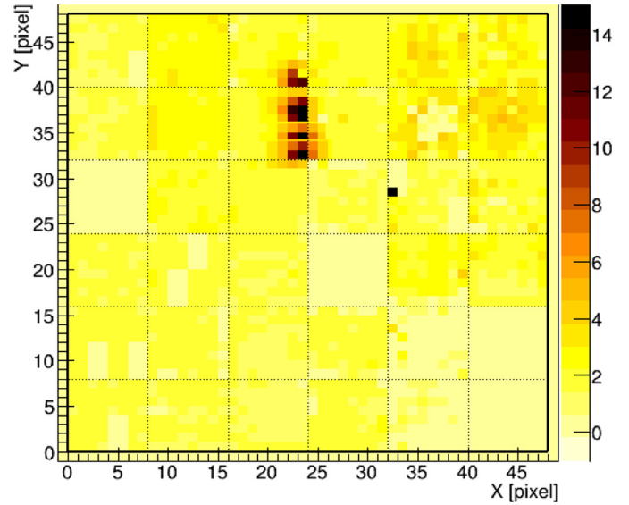
Fig. 12. A meteor track detected by EUSO-TA on the night 12th November, 2015. The picture shows the overlap of four averages of 1280 frames (0.9 s elapsed from the start to the end of the observation, 12.8 ms total integration time). The color scale denotes the uncalibrated detector counts. The apparent magnitude of the meteor in collected data varied from M_B = 2.4 to M_B = 4.06 .
