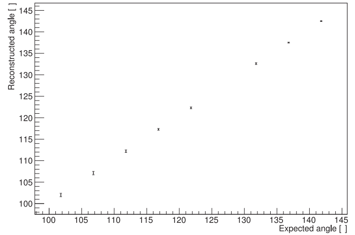
Fig. 18. Reconstructed angle vs expected angle for GLS laser pointing sweep. Barely visible error bars show the standard deviation of the distribution of reconstructed angles.
