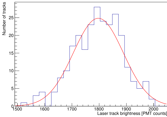
Fig. 16. The reconstructed distribution of the integrated number of counts from 259 CLF shots. The standard deviation of the fitted Gaussian function is about 5%, comparable to the overall intrinsic CLF energy dispersion of 6%.
