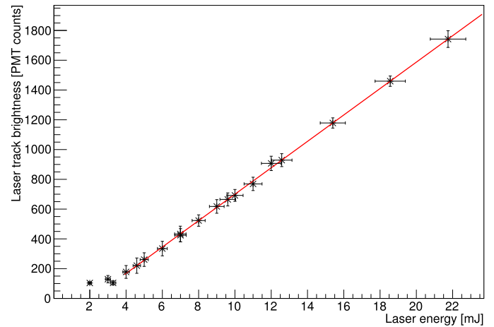
Fig. 19. Summed signal of the GLS laser track vs its energy for the distance of 33 km from the detector. The plot sums 2 shooting sessions, altogether encompassing an energy range of 2–22 mJ. Each point was calculated from a few dozens shots. Fitted line shows good linearity of the detector response in the range of 4–22 mJ, while for lower energies only the brightest tracks were reconstructed, enforcing a low brightness cut on the data points.
