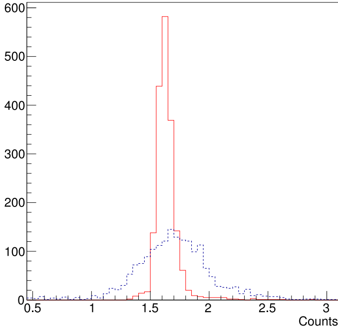
Fig. 9. Histogram of sky background pixel counts on an average of 12,800 frames before (dashed) and after (solid) flat fielding.
