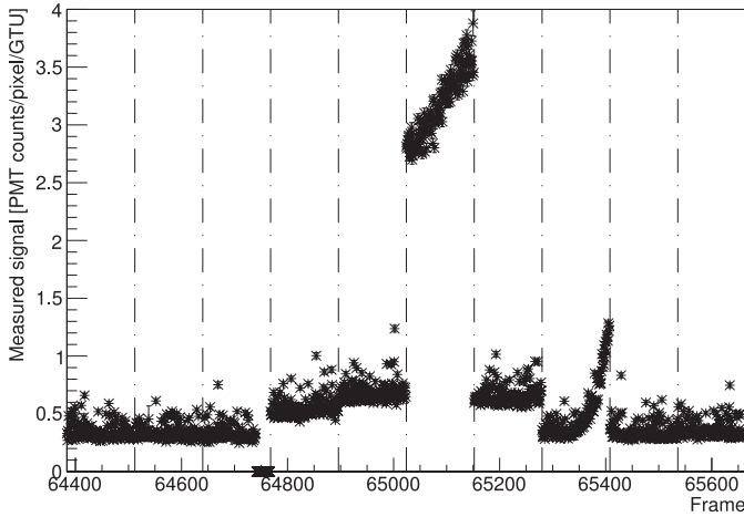
Fig. 13. The lightcurve of the average number of counts per 2.3 \mu s on the whole PDM during a thunderstorm passing close by. The lightcurve is not continuous. Vertical lines show the transition between packets of data. Each packet is a continuous acquisition encompassing 320 \mu s, however the time between packets depends on incoming triggers and in this case was of order of dozens of milliseconds.
