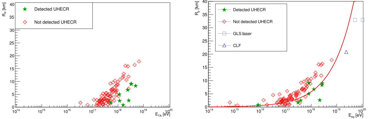
Fig. 20. All UHECR detected by TAFD in the EUSO-TA field of view during its operation with non-detected events and laser shots superimposed. The vertical axis shows the distance to the shower axis. Left: the horizontal axis shows the energy of the event as measured by TA. Right: the horizontal axis shows the events equivalent energy (explained in the text). The fit to the detected points, explained in the main text, suggests a conservative estimate of the EUSO-TA detection energy threshold.
