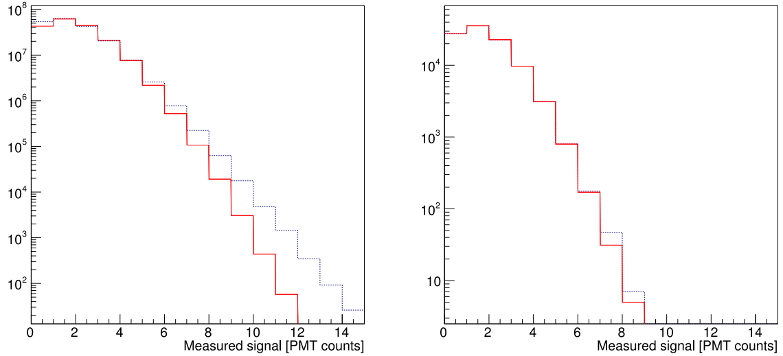
Fig. 6. Left: histogram of counts in all working pixels of the focal surface from 100,000 frames (dashed) and a fitted Poisson distribution (solid), for sky background observations on the night of 16th of May, 2015. Right: similar histogram consisting of counts in a single pixel.
