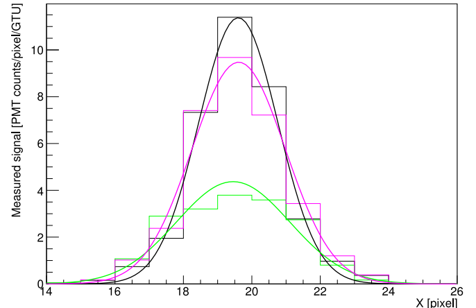
Fig. 17. Left: the width of the CLF averaged track in each row (elevation), measured as a FWHM of a fitted Gaussian profile; Right: horizontal cross-sections of the CLF track. Three histograms show cross-sections in Y positions corresponding to the largest, smallest and intermediate widths, with fitted Gaussian profiles.
