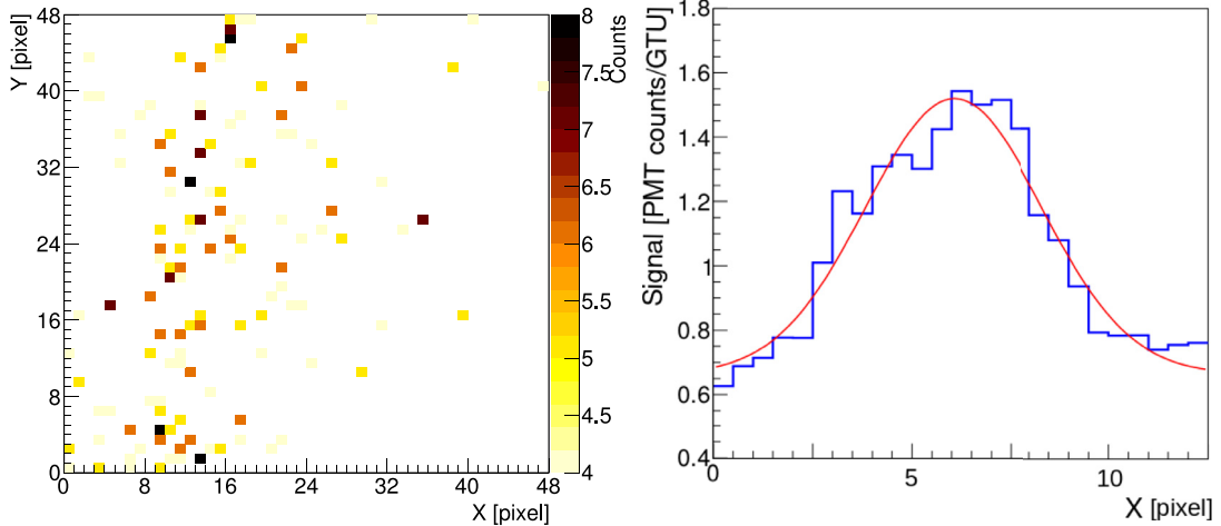
Fig. 22. Left: Residues of the data subtracted from simulation for the second UHECR shown in Fig. 21. The colour scale, in detector counts, is set to emphasise the part including the shower; Right: transversal profile of the same UHECR with subpixel resolution, corrected for the EAS non-vertical axis (the correction causes shift of the maximum compared to the original shower axis and X axis crossing point). The Gaussian fit gives FWHM of 5.27 pixels.
