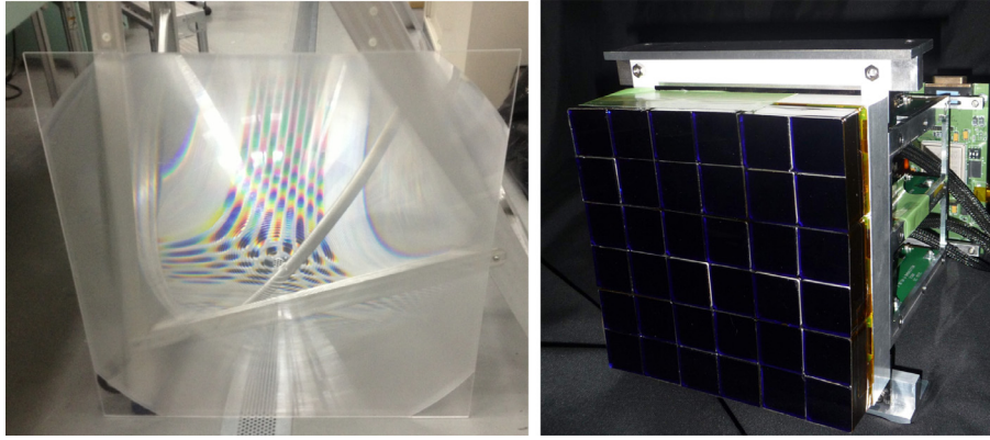
Fig. 4. Left: front 1 m 2 lens of EUSO-TA; Right: the PDM array of side 17.3 cm, composed of 36 MAPMTs, 64 channels each. Behind it 6 ASIC boards are mounted on the PDM frame connected to the PDM board.
