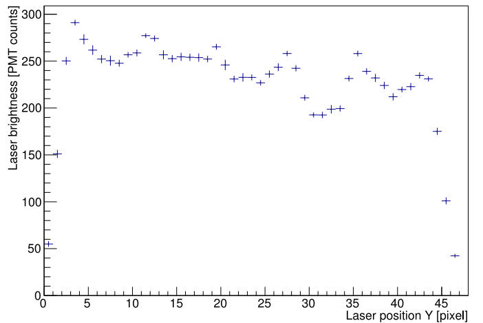
Fig. 15. A profile histogram of 259 CLF laser tracks, for telescope elevation angle of 10^\circ . The values show the average of summed counts for laser spots in a specific position on the frame. The brightness is lower for spots falling into space between MAPMTs or outside the PDM.
