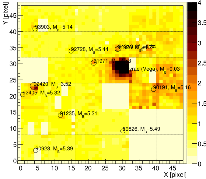
Fig. 10. Sum of 1280 frames acquired with EUSO-TA with the position of the brightest stars superimposed, using the Hipparcos catalogue. Each star is labelled with the catalogue number or the star name in case of Vega, followed by the star's magnitude in the Johnson B filter for objects of M_B \leq 5.5 . The colour scale denotes the brightness of each pixel in arbitrary units after flat fielding. Zero values (bright color) correspond to non-functioning pixels.
