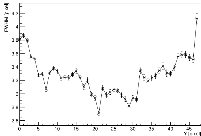
Fig. 17. Left: the width of the CLF averaged track in each row (elevation), measured as a FWHM of a fitted Gaussian profile; Right: horizontal cross-sections of the CLF track. Three histograms show cross-sections in Y positions corresponding to the largest, smallest and intermediate widths, with fitted Gaussian profiles.
