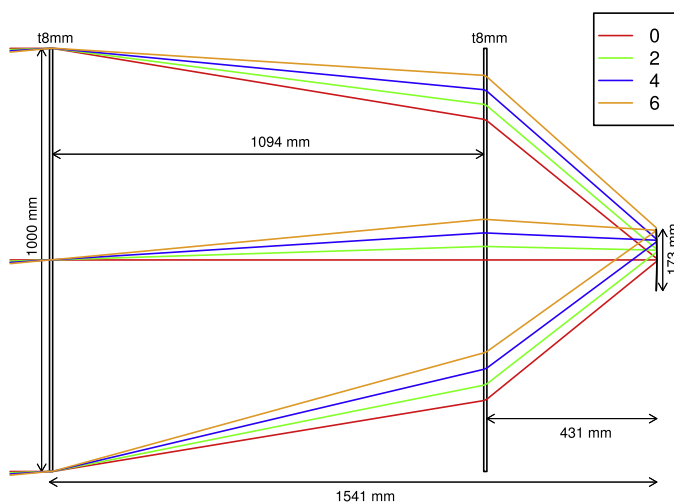
Fig. 3. The design of the EUSO-TA optics. The ray tracing is shown for different incident angles of 0°, 2°, 4° and 6°, respectively.
