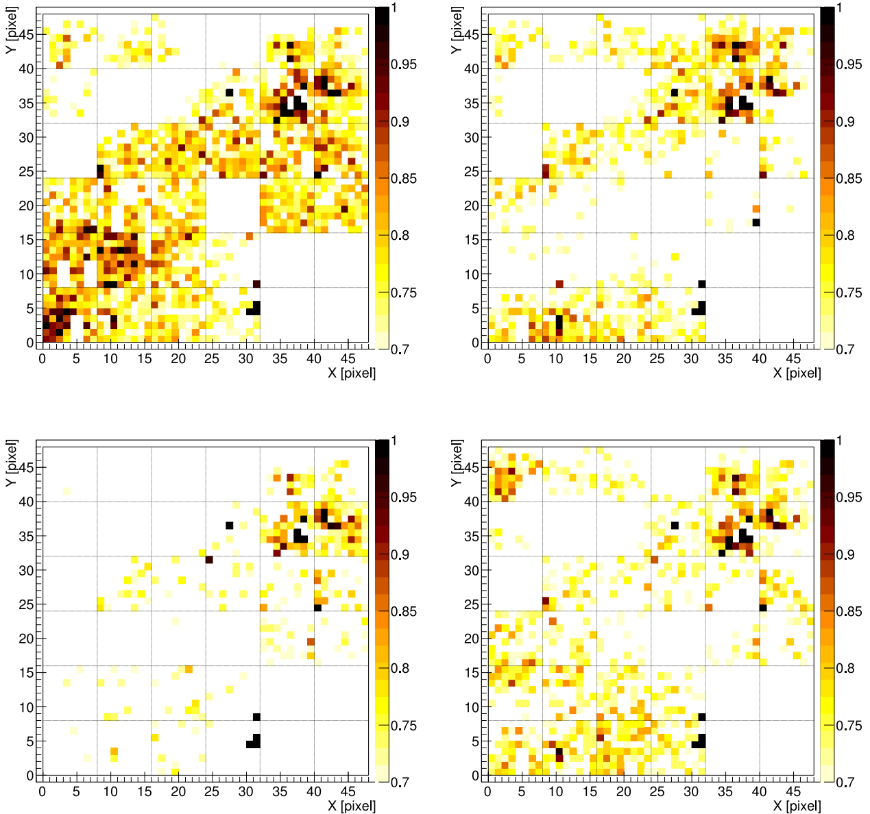
Fig. 8. Examples of clouds (dark areas) passing through the focal surface. The four pictures show averages of 1280 frames separated by a few minutes. The colour scale denotes the brightness of each pixel in arbitrary units after flat fielding. This and all the following figures of this kind show the view of the observer standing behind the instrument and looking at the same part of the sky.
