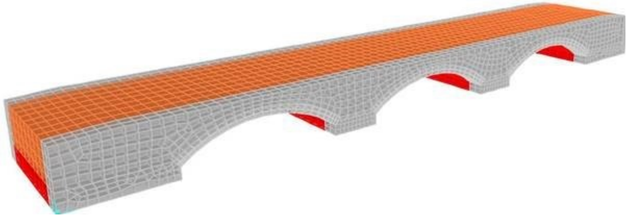
Figure 4: FEM model of Porta Napoli bridge
