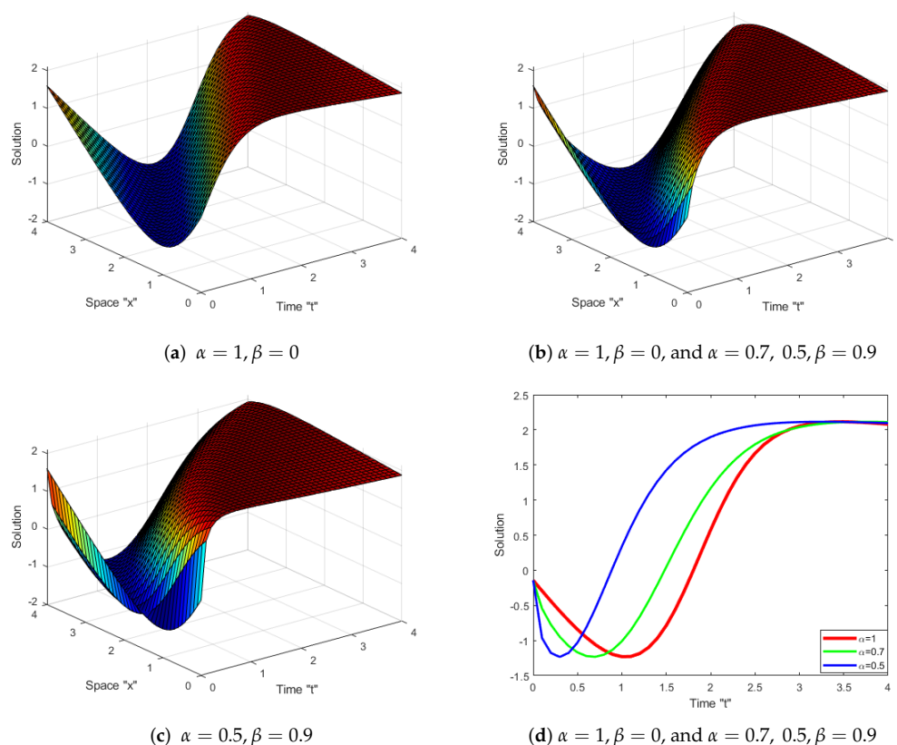
Figure 2. (a–c) identify the 3D profile of Equation (40) (d) denotes the 2D plot for various values of \alpha at x = 1 , and each solution curve is completely distinct from every other one.
