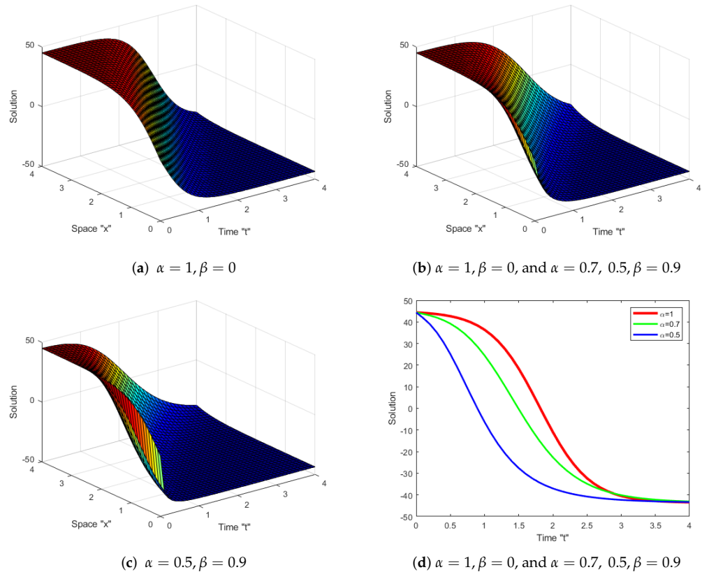
Figure 1. (a–c) identify the 3D profile of Equation (38), (d) denotes the 2D plot for various values of \alpha at x = 1 , and each solution curve is completely distinct from every other one.
